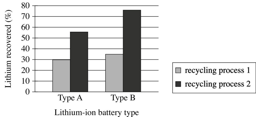
Test Results for Two New Battery Recycling Processes
